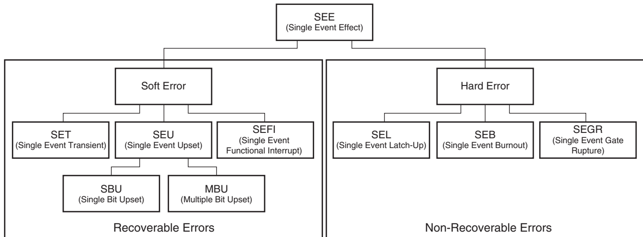
Figure 1: Types of Single Event Effects
