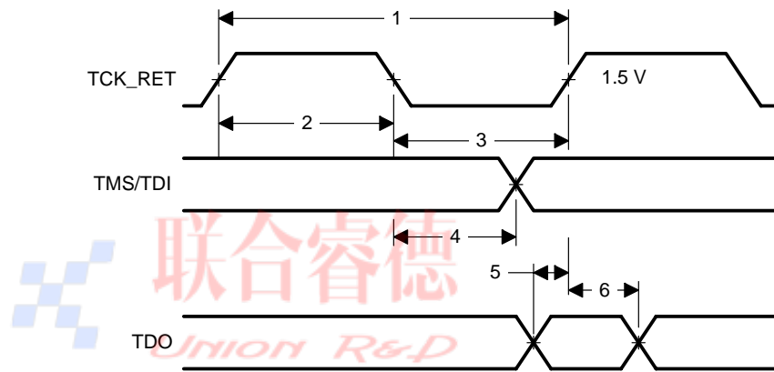
Figure 1–3. JTAG Emulator Cable Pod Timings
