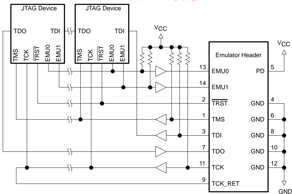
Figure 1–5. Multiprocessor Connections
